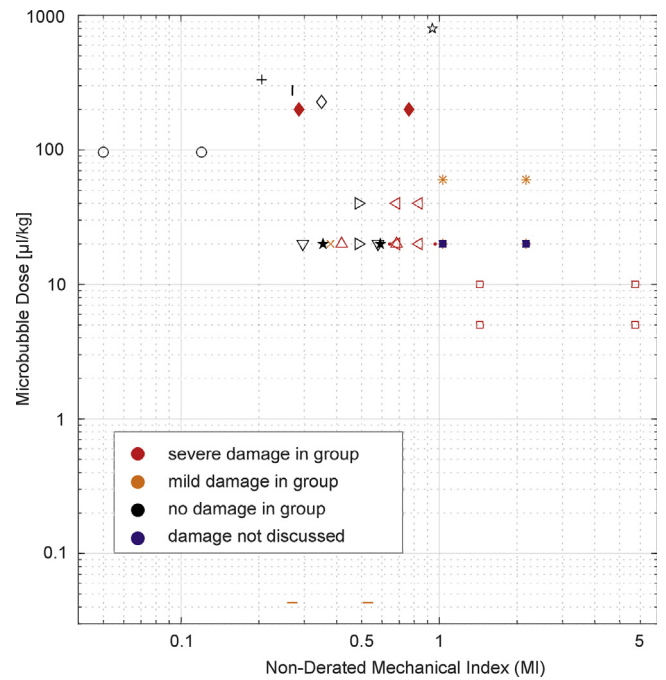
Figure 7. Blood–spinal cord barrier opening studies plotted against the non-derated mechanical index (MI) and the microbubble dose. Red denotes ultrasound-induced damage, yellow denotes damage caused by other means or minor damage, black denotes no damage, blue denotes studies in which damage was not discussed. o , Shimamura et al. 2005 [10]; + , Takahashi et al. 2007 [11]; – , Wachsmuth et al. 2009 [88]; ◁ , Oakden et al. 2014 [141]; × , Weber-Adrian et al. 2015 [13]; | , Song et al. 2017 [14]; * , Payne et al. 2017 [91]; ◊ , Song et al. 2018 [15]; ∇ , O’Reilly et al. 2018 [16]; ◆ , Montero et al. 2019 [25]; • , Fletcher et al. 2019 [89]; ▷ , → Shah 2020 [17]; □ , Fletcher et al. 2020 [90]; ★ , Smith et al. 2021 [18]; ■ , Cross et al. 2021 [92]; △ , Fletcher et al. 2021 [87]; ☆ , Bhimreddy et al. 2023 [93].
