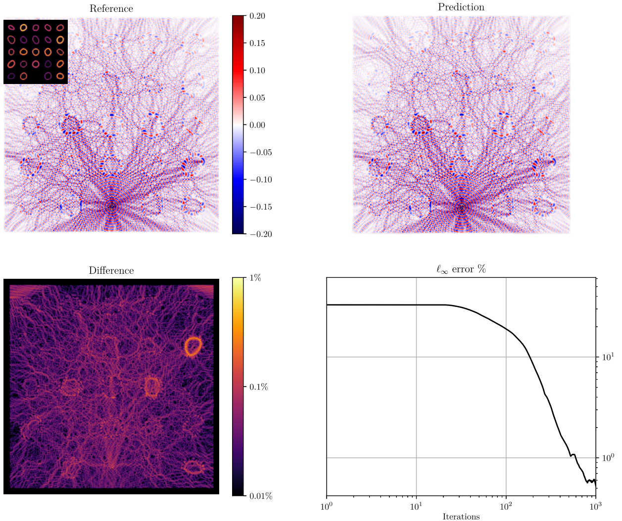
Fig. 11. Test on a spatial domain much larger than that seen during training. The sound speed distribution is created by patching together 24 idealized skull distributions from the test set (inset top left). The reference solution is computed using k-Wave and shows very close agreement with the prediction using the learned optimizer, with errors well below 1% (the real part of the wavefield is shown). The relative \ell_\infty error against the reference solution takes approximately 600 iterations to reach 1%.
