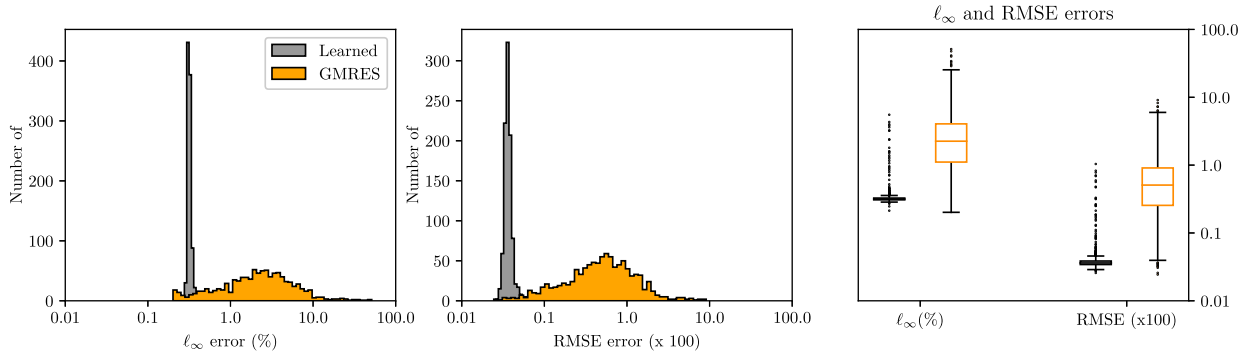
Fig. 5. Errors in the wavefields predicted by the learned optimizer and the generalized minimal residual (GMRES) method shown as histograms (left and middle) and box plots (right). The errors are compared after 1000 iterations against a reference solution calculated using k-Wave for the 1000 sound speed distributions in the test set. The plotted RMSE errors are multiplied by 100 to move them to a similar scale. The learned optimizer is highly accurate, with a mean \ell_\infty error of 0.36%, and mean root mean square error (RMSE) of 4.6 \times 10^{-4} .
