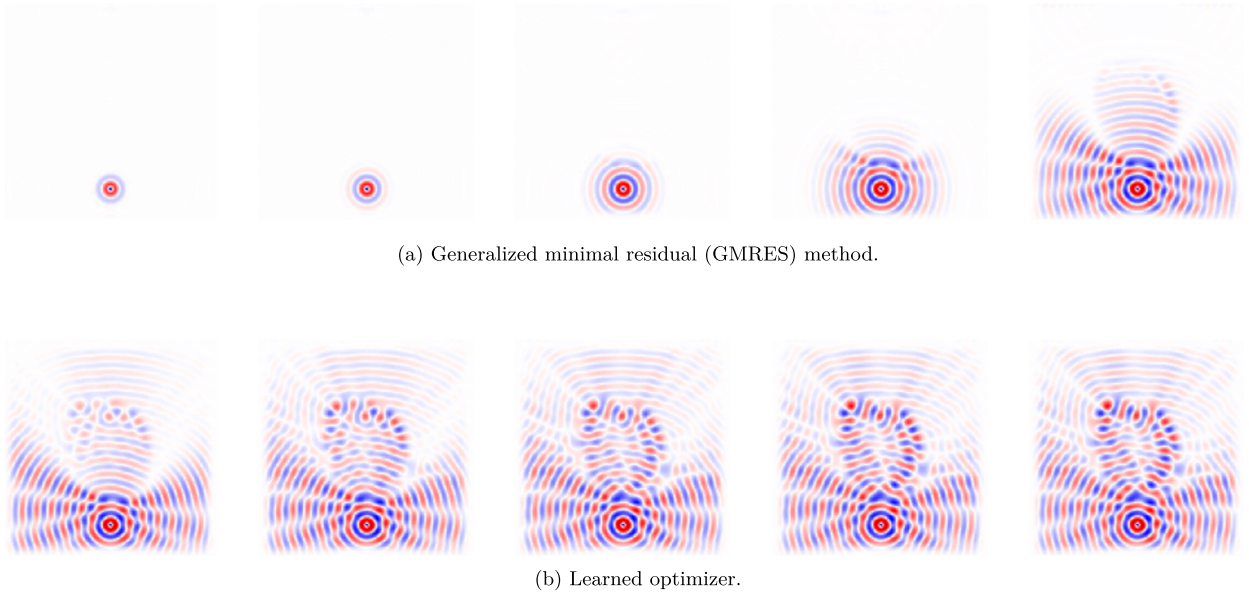
Fig. 9. Evolution of the solution after 10, 20, 50, 100, and 250 iterations for GMRES and the learned optimizer for a sound speed distribution from the test set (the real part of the wavefield is shown). The results for GMRES demonstrate the local nature of Krylov iterations based on the Helmholtz operator, which build the solution from the source location outwards. The results for the learned optimizer show a similar dynamic, but the updates cover the global domain much more rapidly.
