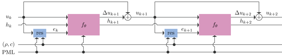
Fig. 2. Schematic of the proposed iterative scheme (showing two iterations) for the solution of the heterogeneous Helmholtz equation u . This uses a fully-learned optimizer f_\theta which outputs both the solution update \Delta u_k along with a belief state h_k . The residual e_k is calculated using a physics loss (represented in the figure by the block res). This is different for every speed of sound distribution and is used as an additional input to the network. Both the optimizer and the residual calculation make use of knowledge of the perfectly matched layer (PML). The residual calculation also uses the sound speed c and source distribution \rho through the forward operator.
