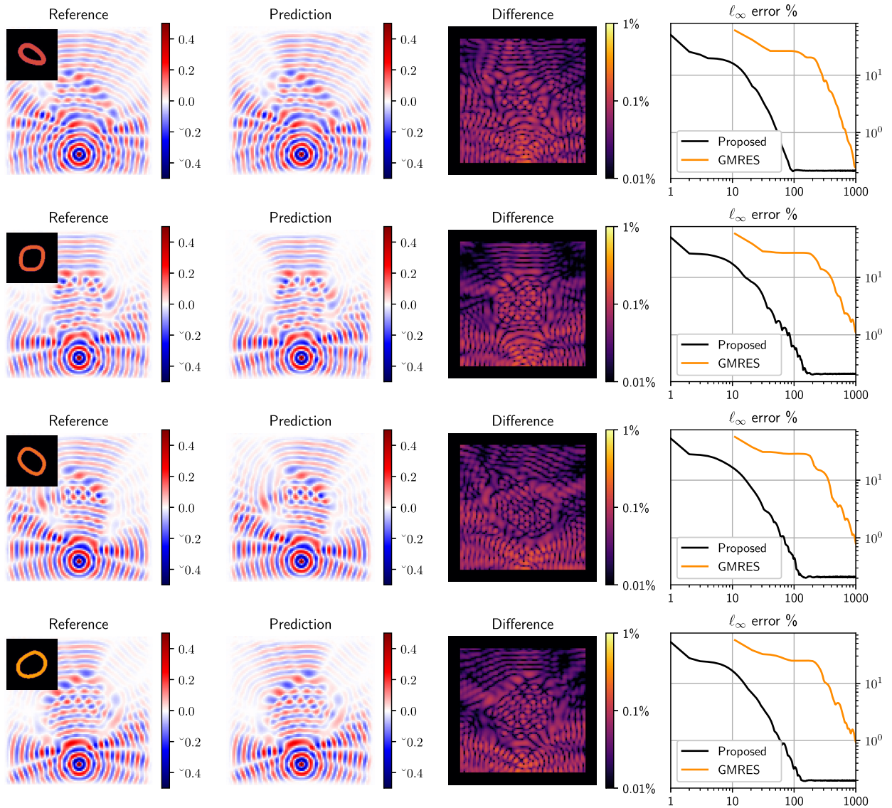
Fig. 6. Four examples of simulations using idealized skull distributions randomly selected from the test set (insets shown top left). In each case, the reference solution is computed using k-Wave and shows very close agreement with the prediction using the learned optimizer (the real part of the wavefield is shown). For these examples, the \ell_\infty error reaches a minimum within 200 iterations. The convergence of GMRES is also shown for comparison: we reset the Krylov subspace every 10 iterations.
