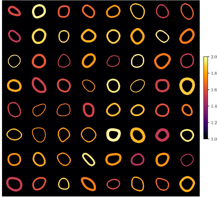
Fig. 4. Examples of the sound speed distributions based on idealized skulls used to train the learned optimizer. Each skull is created by summing up several circular harmonics of random amplitude and phase, and then assigned a random thickness between 2 and 10 pixels, and a random sound speed between 1.5 and 2 times the background value. (For interpretation of the colors in the figure(s), the reader is referred to the web version of this article.)
