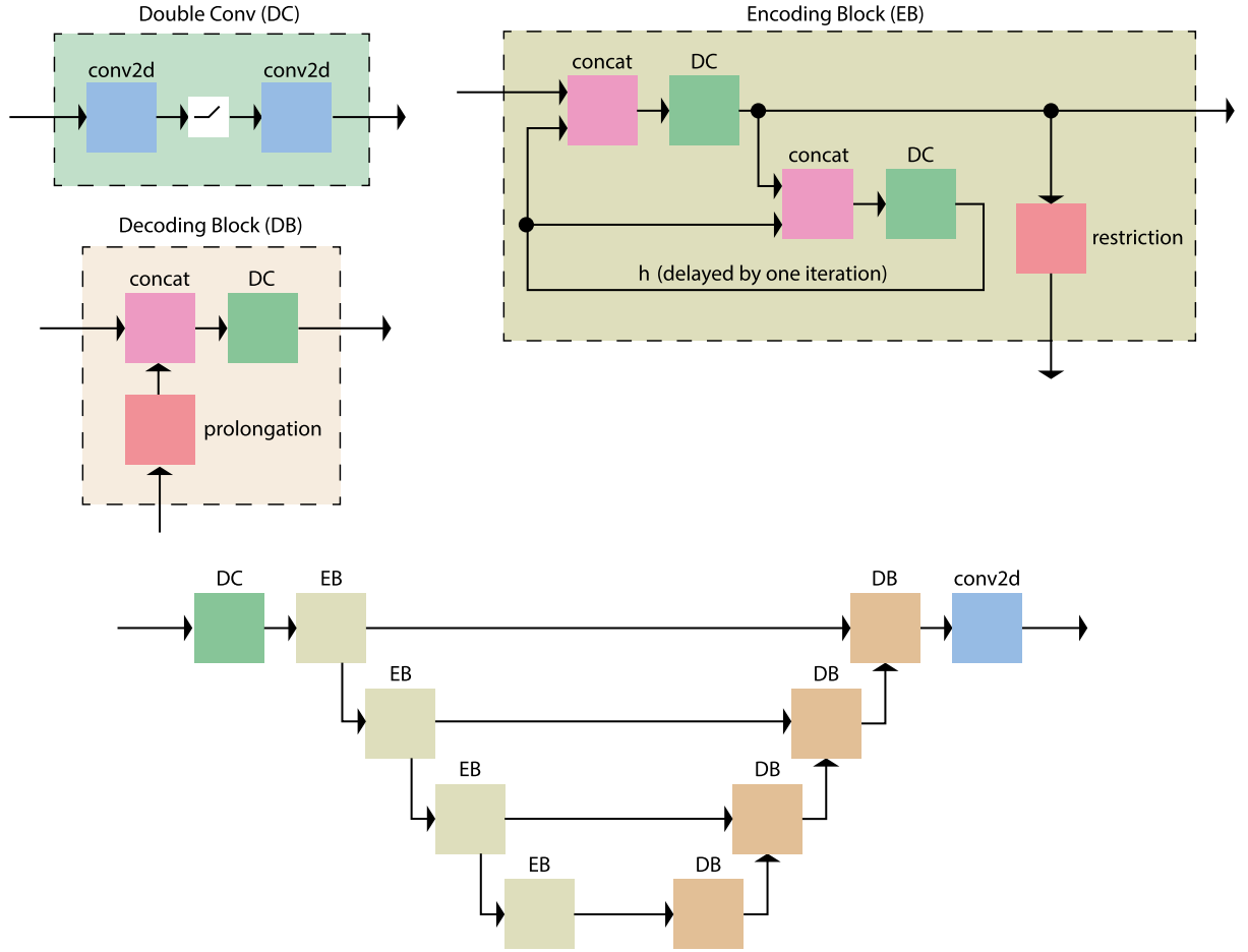
Fig. 3. Architecture of the modified UNet used for the learned optimizer f_\theta . Each encoding block (EB) contains two double convolution (DC) layers, one to compute the output passed to subsequent layers, and one to compute the hidden state h . The concat blocks stack the inputs in the channel dimension. The network is lightweight, with only 8 channels per convolutional block at every scale and a total of 47k trainable parameters.
