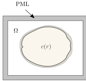
Fig. 1. Definition of the computational domain \Omega which contains a heterogeneous sound speed c(r) , in this case represented by a skull. A perfectly matched layer (PML) is used to surround the computational domain to simulate exterior open boundaries as discussed in Appendix A.
