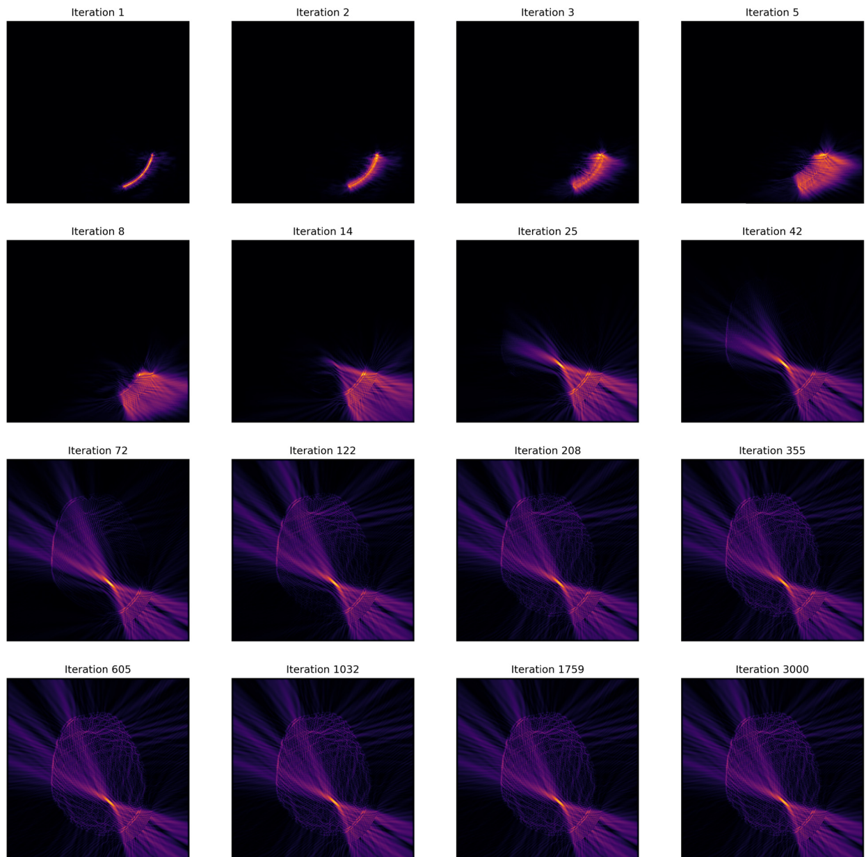
Fig. 13. Evolution of the wavefield predicted by the learned optimizer for different iteration numbers for the transcranial ultrasound example given in Fig. 12. The position of the focus and the focal pressure converge with 20 iterations, and most of the complex structure in the field can be seen after just 200 iterations. Note, the colormap of each subpanel is normalized by its own maximum.
