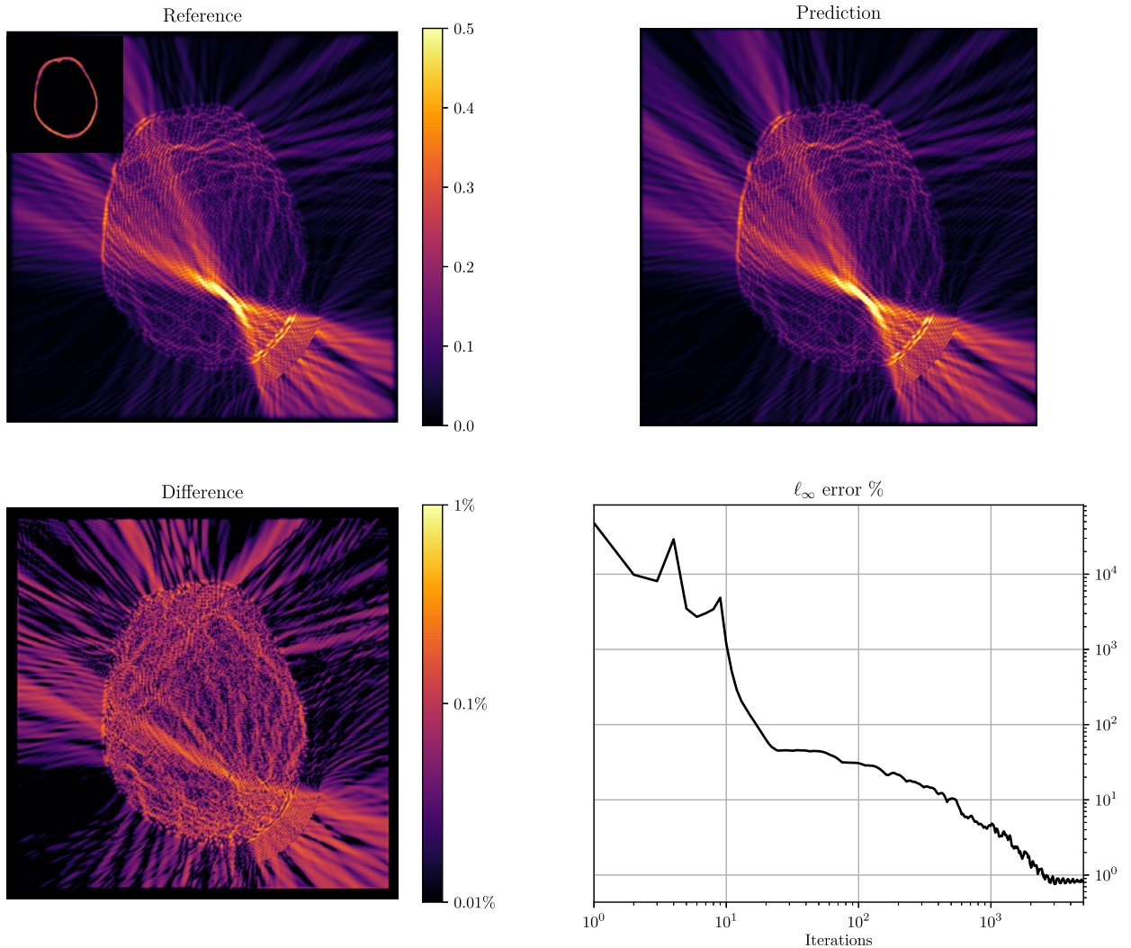
Fig. 12. Simulation of a transcranial ultrasound field using a sound speed distribution generated from a clinical x-ray computed tomography (CT) slice (inset top left). The reference solution (top left) is computed using k-Wave and shows very close agreement with the prediction using the learned optimizer (top right), with errors below 1% (bottom left). The absolute value of the complex wavefield is shown. The \ell_\infty error takes approximately 3000 iterations of the optimizer to reach a minimum (bottom right).
