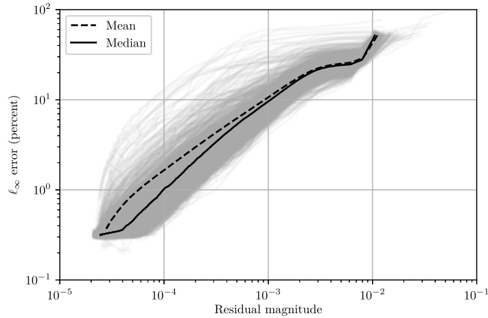
Fig. 7. Trajectories showing the evolution of the \ell_\infty error against the residual loss for the 1000 sound speed distributions in the test set. The \ell_\infty error is calculated by comparison with k-Wave, and the residual is calculated using a physics loss term. The dashed and solid lines indicate the mean and the median of all traces, respectively.
