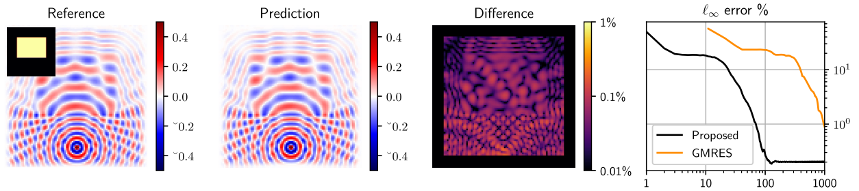
Fig. 10. Simulation using a large rectangular heterogeneity (inset top left) which has a shape unlike the speed of sound distributions seen during training. The reference solution is computed using k-Wave and shows very close agreement with the prediction using the learned optimizer (the real part of the wavefield is shown). The relative \ell_\infty error against the reference solution takes approximately 70 iterations to reach 1%.
