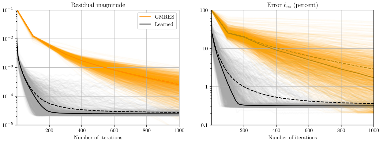
Fig. 8. Progression of the optimization problem with the number of iterations for the learned optimizer (black) and the generalized minimal residual (GMRES) method (orange) for the 1000 sound speed distributions in the test set. The dashed and solid lines indicate the mean and the median of the individual traces, respectively. (left) Magnitude of the residual. (right) \ell_\infty error compared to k-Wave.
