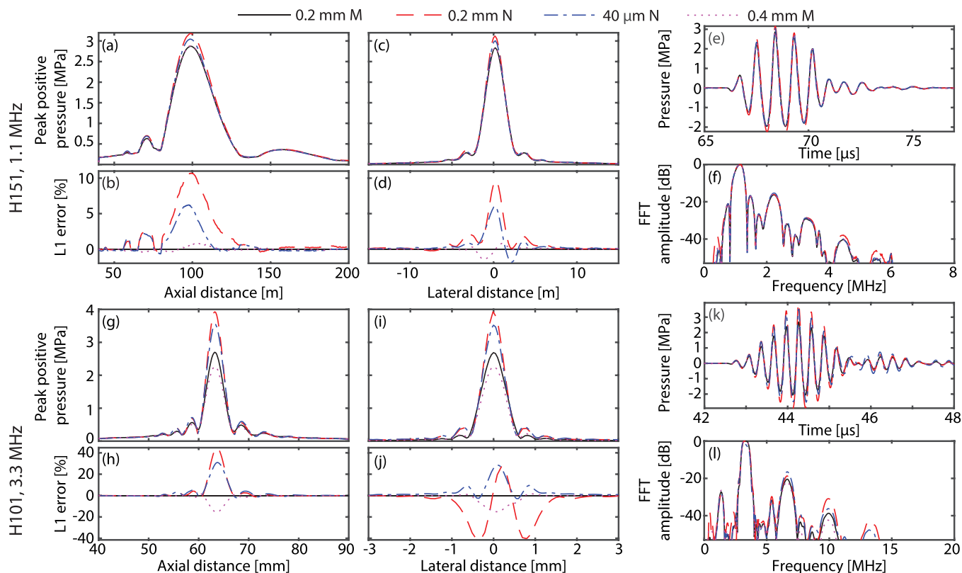
FIG. 5. (Color online) Measurements of the field of single element bowl transducers in pulsed mode made with the four test hydrophones. For H151 at 1.1 MHz: (a) Axial peak positive pressure and (b) L_1 error at each scan point. (c) Lateral peak positive pressure and (d) L_1 error at each scan point. (e) Focal waveforms and (f) spectra. For H101 at 3.3 MHz: (g) Axial peak positive pressure and (h) L_1 error at each scan point. (i) Lateral peak positive pressure and (j) L_1 error at each scan point. (k) Focal waveforms and (l) spectra. M: membrane, N: needle.
